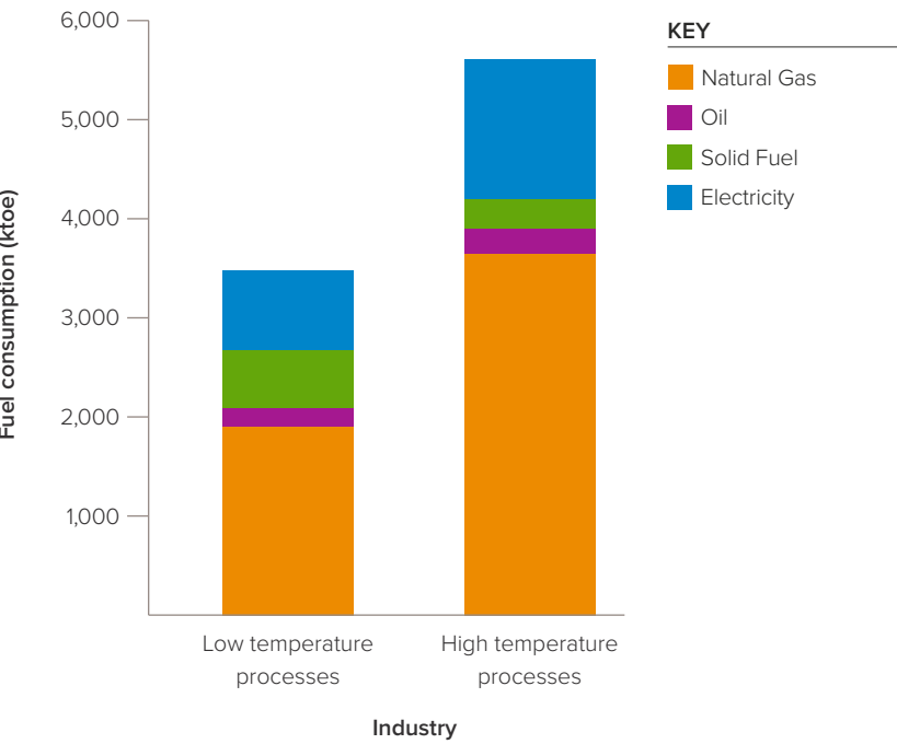
UK industry process heat consumption by fuel (2018) 37 .
